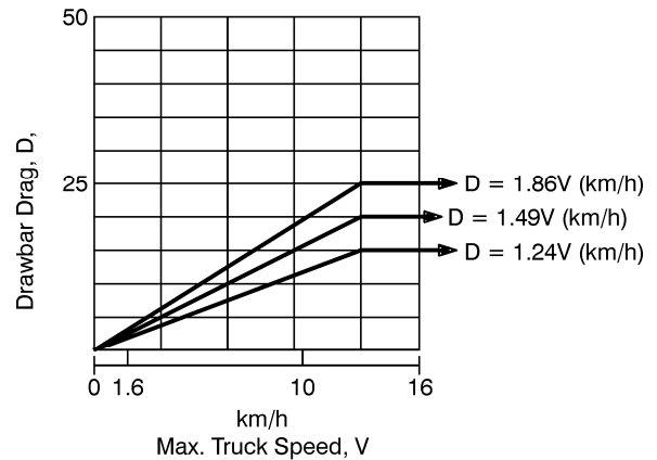
Fig. 2 Service Brake Performance Requirements
