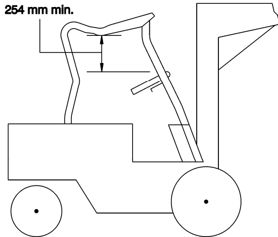
Fig. 6 Overhead Guard Impact Deformation Limit (Sit-Down)
